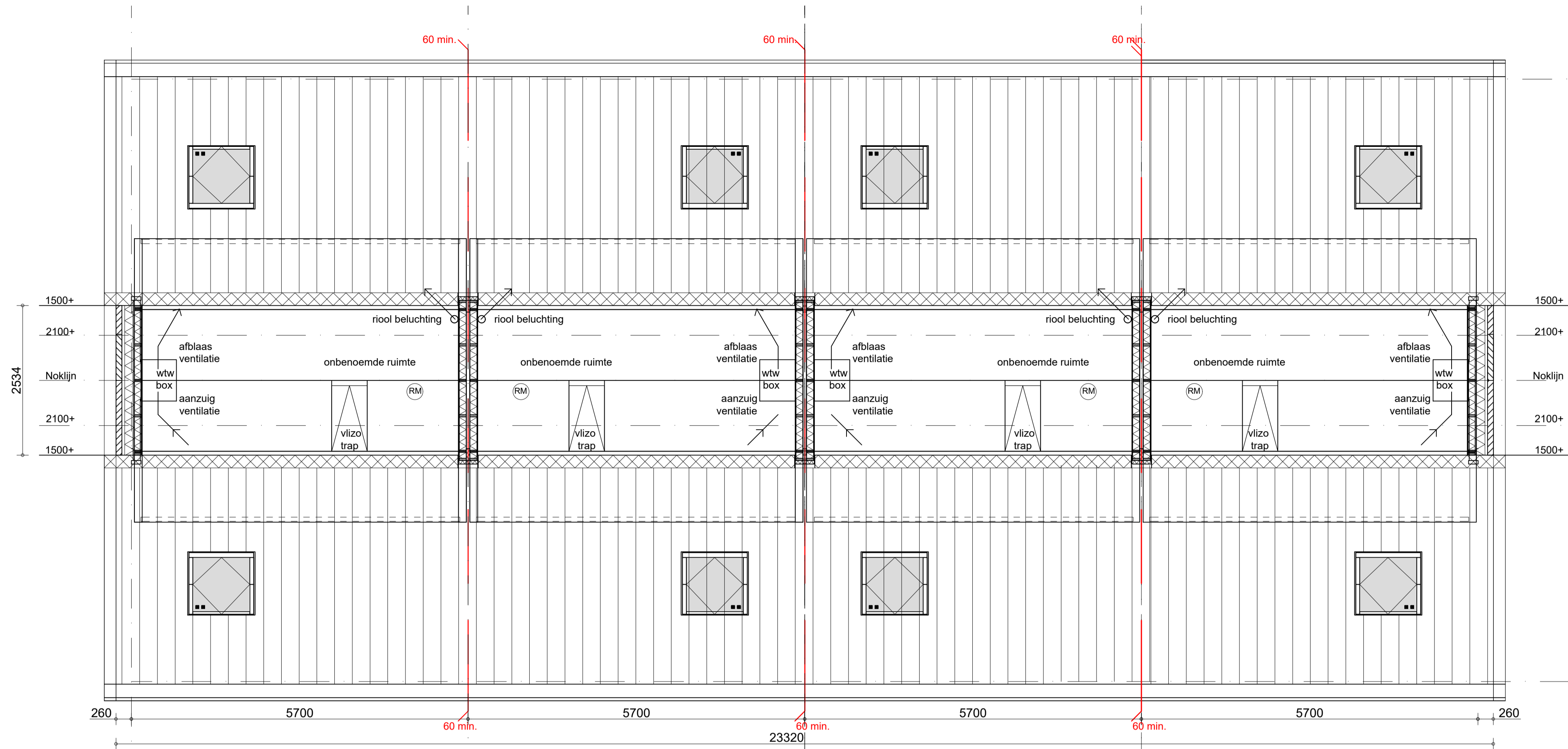
Zolder 1:50
