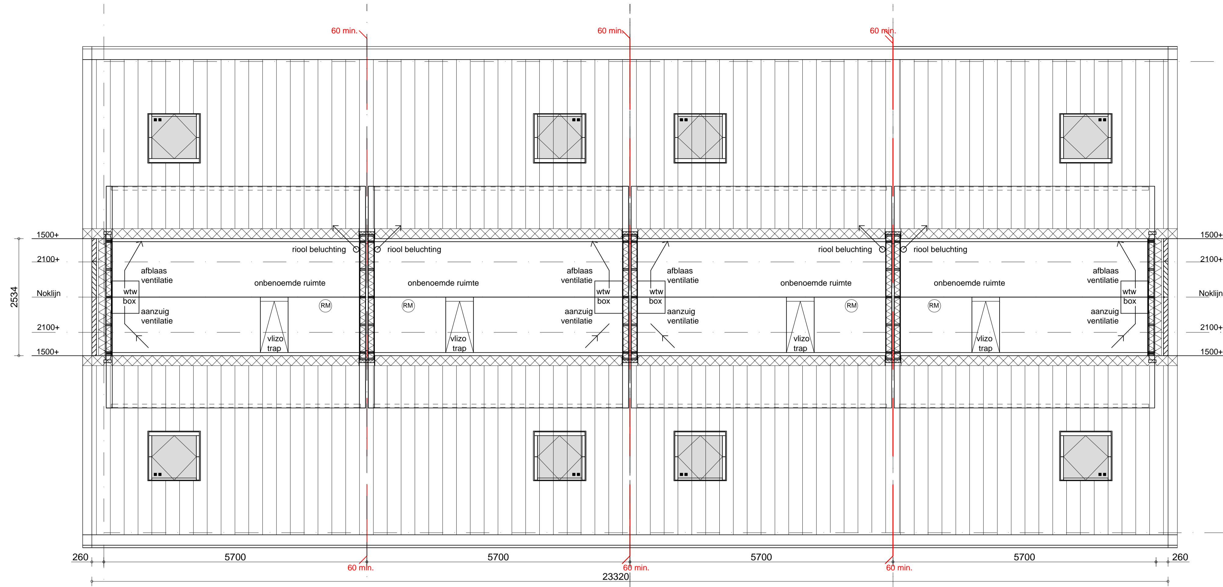
Zolder 1:50
